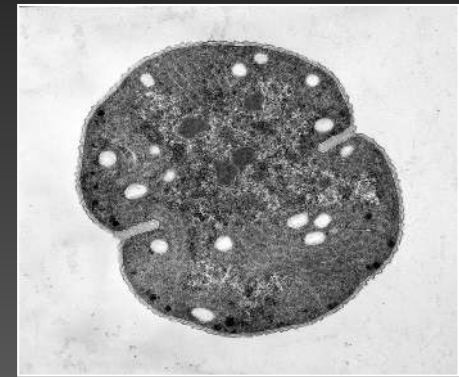
Crococosphera
