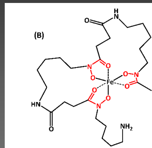
Desferrioxamine B
