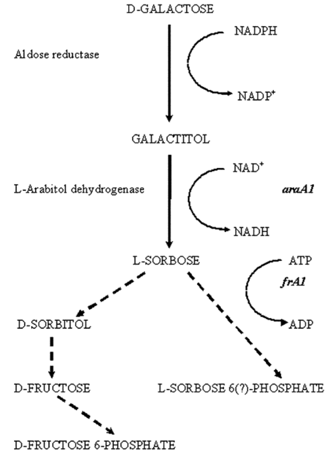
Fig. 8 The reductive D-galactose degrading pathway. Broken lines Alternative catabolic pathways
