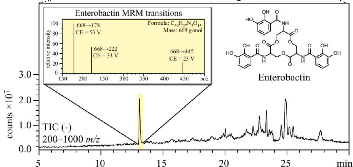
HPLC-MS chromatogram
