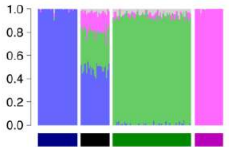
Recent admixture into Ari Cultivators
