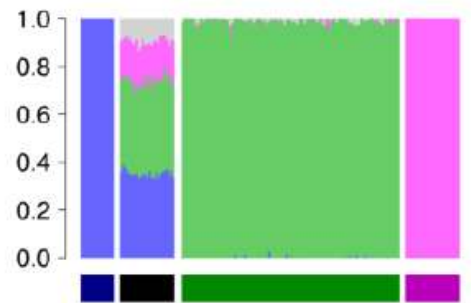
Strong drift in Ari Blacksmiths
