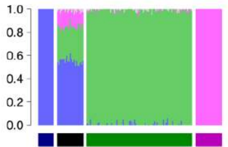
Ghost admixture into Ari Cultivators
