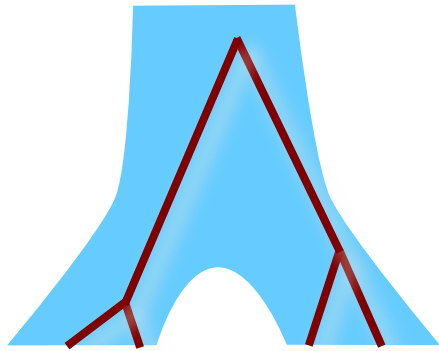
First Coalescence within Population 1
