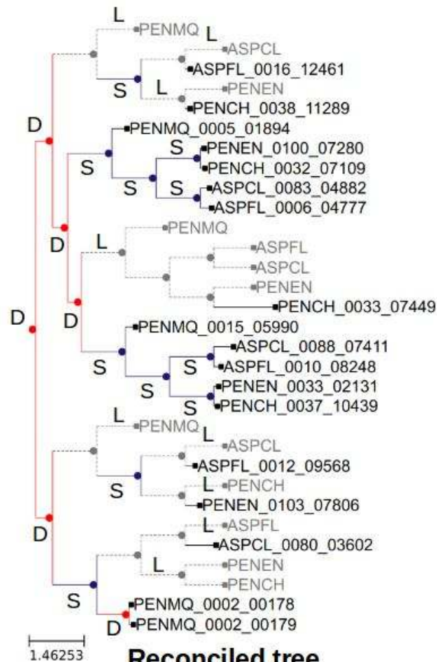
Reconciled tree
