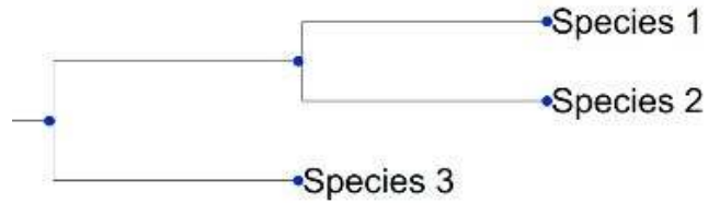
Species tree
