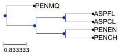
Species tree
