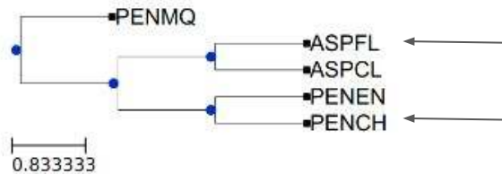
Species tree
