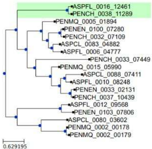
Gene tree
