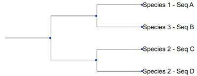
Gene tree
