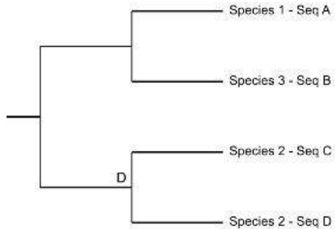
Species overlap
