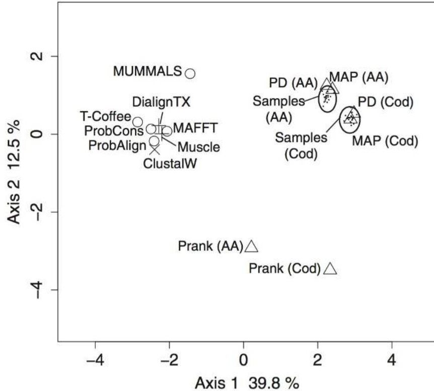
Fig. 1. Blackburne & Whelan. 2013. Mol. Biol. Evol. 30(3):642–653.
