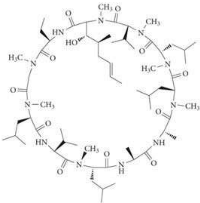
Cyclosporine A
