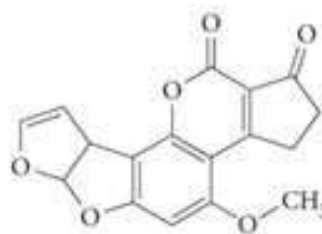
Aflatoxin B1
