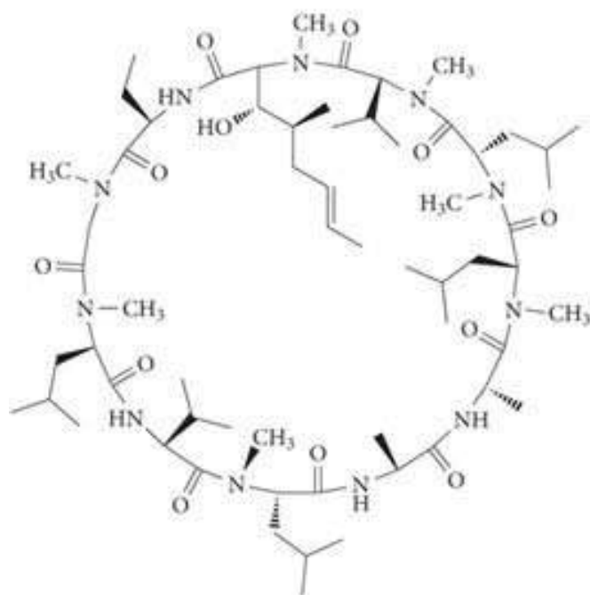
Cyclosporine A
