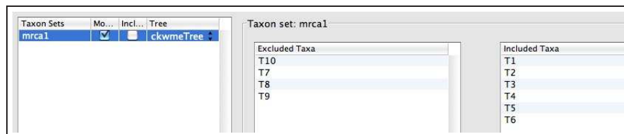
Figure 9: Defining the taxon set for the most recent common ancestor of T1, T2, T3, T4, T5, and T6.
