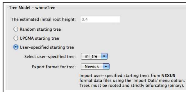
Figure 14: Specifying a starting tree.
