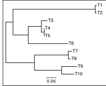
Figure 4: A maximum likelihood estimate of the phylogenetic relationships of ckwme.nex . (Constructed using PAUP* v4.0a125; Swofford, 1998)
