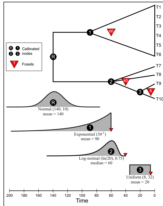
Figure 5: Four nodes with fossil calibration for the ckwme.nex data set. There are calibrations on the root and 3 other internal nodes. Each calibration point is assumed to have a different prior density.
