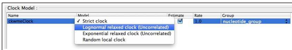
Figure 11: Options for modeling among-lineage substitution rate variation in the Clock Model menu.
